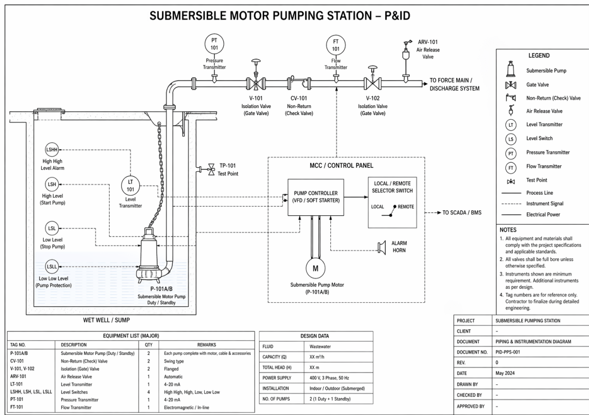
Figure 2: Submersible Motor Pumping Station PID Diagram
